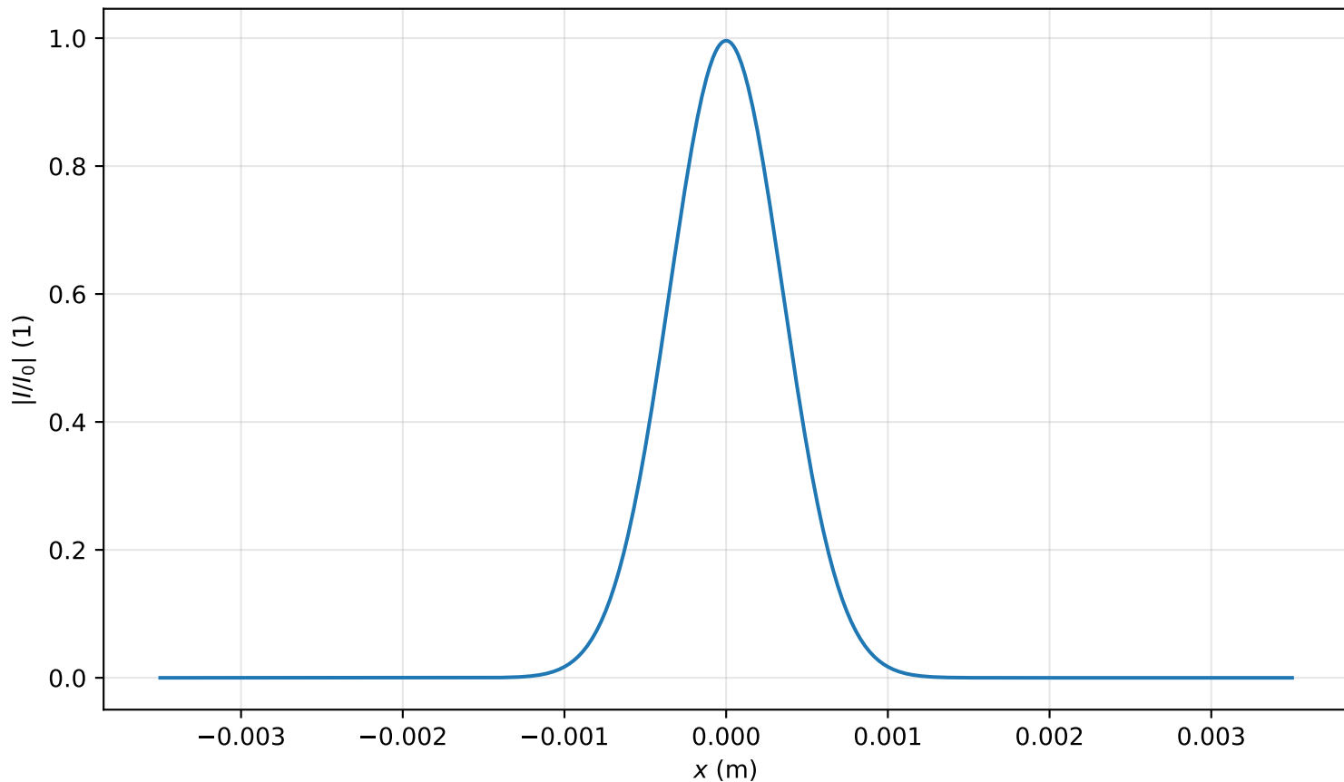
Intensity profile I(x, y = 0, z = 0.159m)/I_0 , P_{in}=0.1P_{cr} , artificial time
